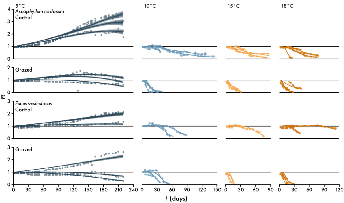
1000 Figure 6. Example 5: the effect of temperature and grazing on the decomposition of floating 1001 Ascophyllum nodosum and Fucus vesiculosus (n = 1651, data from Vandendriessche et al. 1002 2007). Data are plotted alongside predictions of the mean \bar{m} for each replicate (Equation 20, 1003 cf. Figure S6). Lines and intervals are medians and the central 50, 80 and 90% of posterior 1004 probability.
