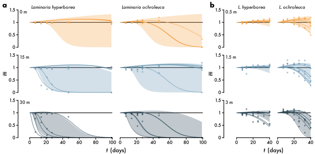
Figure 5. Example 4: the effect of light attenuation with depth on the decomposition of Laminaria hyperborea and Laminaria ochroleuca ex situ ( a , n = 210 , data from Frontier et al. 2021) and in situ ( b , n = 252 , data from Frontier et al. 2022), shown as the proportion of remaining mass over time t . Data are plotted alongside predictions of the mean \bar{m} where lines are medians per replicate and intervals are the central 90% of posterior probability across replicates (Equation 19, cf. Figure S5).
