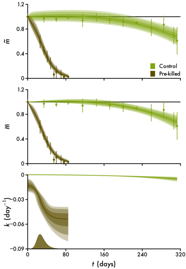
967 Figure 2. Example 1: the effect of physiology on the decomposition of Desmarestia anceps , 968 shown as the proportion of remaining mass (mean \pm standard deviation, n = 5 ) over time t ( n 969 = 115 , data from Brouwer 1996). Data are plotted alongside predictions of new observations 970 \tilde{m} , the mean \bar{m} , the time-variant exponential decay rate k and the photosynthetic half-life \mu 971 (Equation 15, cf. Figure S2). Lines and intervals are medians and the central 50, 80 and 90% 972 of posterior probability. The distribution is a kernel density estimate of the probability density 973 function of \mu .
