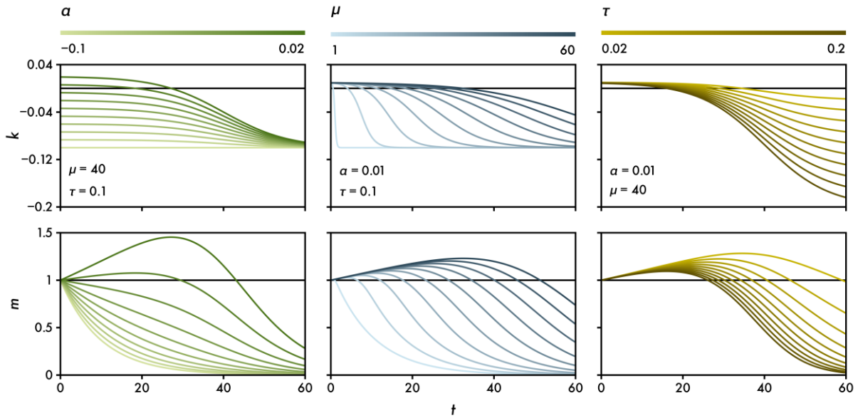
Figure 1. The mathematical model: the effect of varying \alpha , \mu and \tau on the trajectory of the exponential decay rate k (Equation 6) and the proportion of remaining mass m (Equation 9) over time t (cf. Figure S1).
