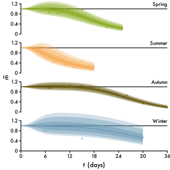
Figure 4. Example 3: the effect of season on the decomposition of Ulvaria obscura ( n = 28 , data from Bourguès et al. 1996). Data are plotted alongside predictions of new observations \tilde{m} (Equation 18, cf. Figure S4). Lines and intervals are medians and the central 50, 80 and 90% of posterior probability.
