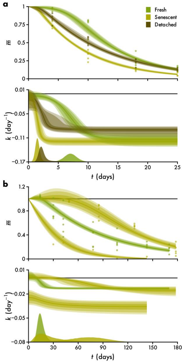
Figure 3. Example 2: the effect of senescence on the decomposition of Macrocyctis pyrifera (a, n = 61, data from Hamersley et al. 2015) and Laminaria hyperborea (b, n = 63, data from de Bettignies et al. 2020), shown as the proportion of remaining mass over time t . Data are plotted alongside predictions of the mean \bar{m} , the time-variant exponential decay rate k and photosynthetic half-life \mu (Equations 16 and 17, cf. Figure S3). Lines and intervals are medians and the central 50, 80 and 90% of posterior probability. Distributions are kernel density estimates of the probability density function of \mu .
